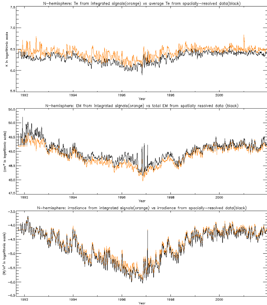
Figure 11. Northern hemispheric coronal temperature (top), emission measure (middle) and irradiance (bottom) obtained from the spatially resolved data (black lines) compared with those from the spatially integrated signals (orange lines). Data points were smoothed by 7-day running average.
