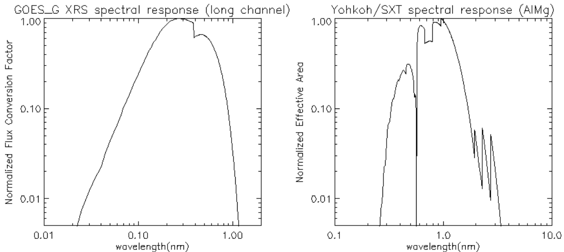
Figure 9. Normalized spectral responses of GOES/XRS long channel and Yohkoh/SXT AIMg filter. The GOES response (left) was prepared from the Calibration Report for XRS ( https://ngdc.noaa.gov/stp/satellite/goes/doc/Document-02(Jan1985)_goesg_xrs_calibration.pdf ), which is identical to the XRS aboard the GOES-7. The flux conversion factor for the B Chamber (0.1-0.8nm) was normalized by its peak value. The SXT response (right) was calculated from the SXT effective area function for the AIMg filter, by normalizing relative to its peak value.
