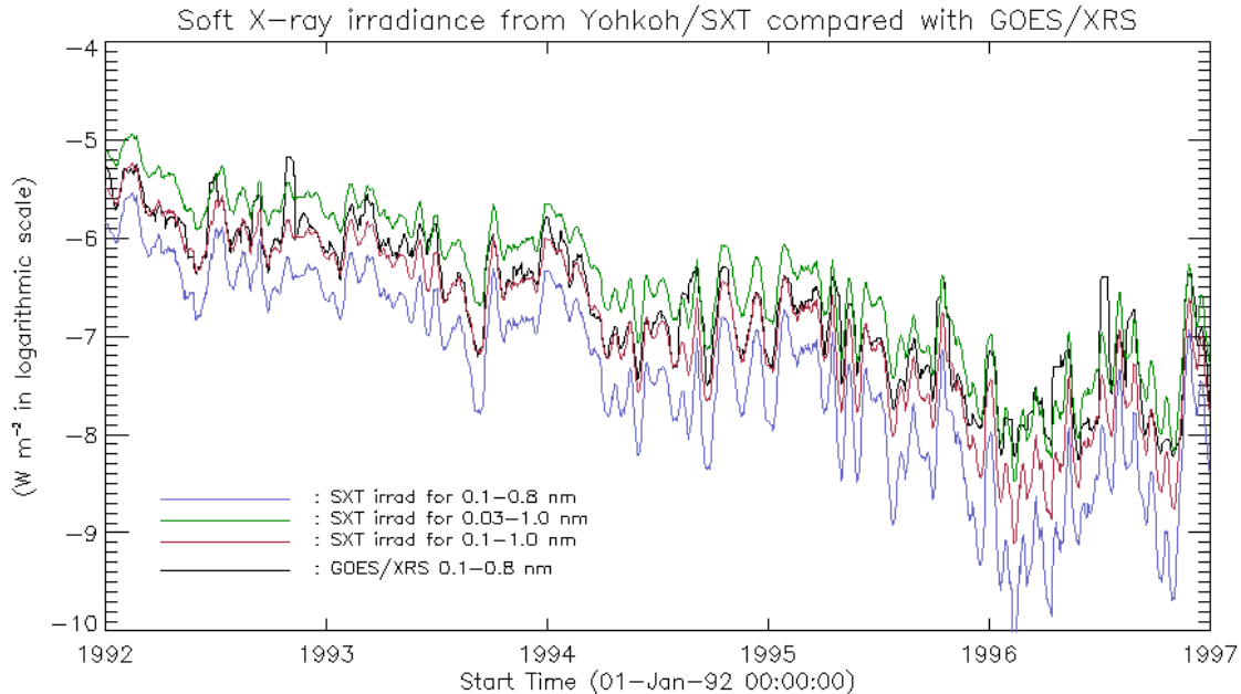
Figure 8. SXT daily averaged irradiances calculated for the wavelength ranges similar to GOES/XRS long channel for the period 1992 to 1997. The wavelength ranges are 0.1 to 0.8 nm (blue line), 0.03 to 1.0 nm (green line) and 0.1 to 1.0 nm (red line), compared with the daily averaged GOES/XRS long channel flux (black line).
