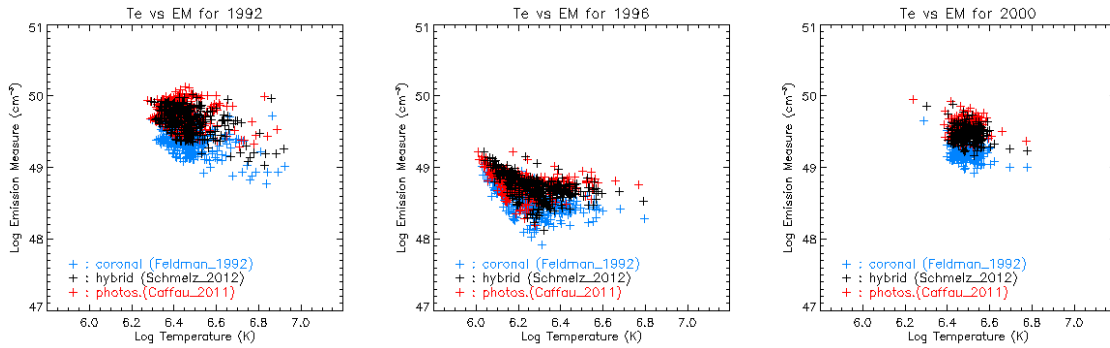
Figure 7. Scatter plot of daily averaged filter-ratio temperatures and emission measures with different elemental abundance assumptions. See the caption of Fig. 6 for convention.
