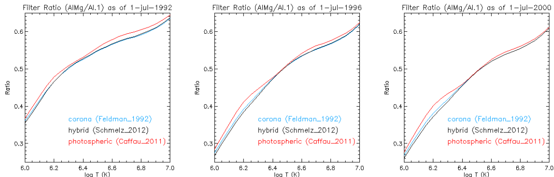
Figure 6. SXT temperature response functions with different elemental abundance assumptions for the year 1992(left), 1996(middle) and 2000(right). The blue, black and red lines denote 'coronal', 'hybrid' and 'photospheric' abundances, respectively.
