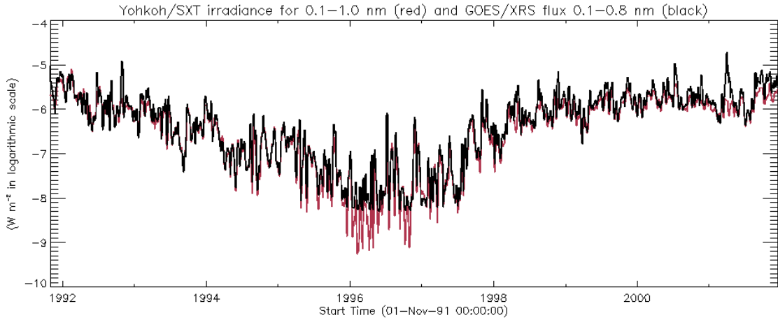
Figure 10. Mission-long variation of the SXT irradiance for 0.1 to 1.0 nm wavelength range compared with the XRS irradiance of the long channel. Both data are daily averaged and smoothed with 14 days window.
