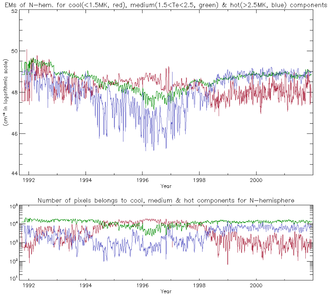
Figure 13. Top plot: Mission-long variation of the emission measures of the cool (red), medium (green) and hot (blue) components of the Northern hemispheric corona. See text for definition. Bottom plot: Variation of the number of pixels that belongs to each temperature component of the above plot. Data points of the both plots were smoothed by 5-day running average.
