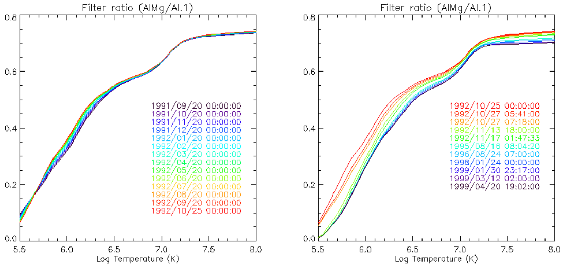
Figure 3. Temporal variation of filter ratio function (AlMg/Al.1), for the same periods as Figure 2.
